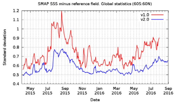
Figure 10: Global [60S; 60N] standard deviation of SMAP SSS – FOAM SSS for the 0.25^{\circ} \times 0.25^{\circ} L3 8-day running averages maps. Red: V1.0 (BETA). Blue: V2.0. Provided by J. Martínez, BEC.
