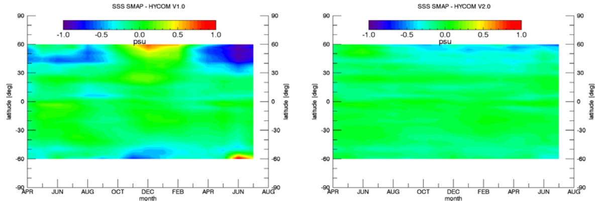
Figure 13: Seasonal distribution of zonally averaged biases between SMAP and HYCOM SSS. Left: V1.0 (BETA). Right: V2.0.
