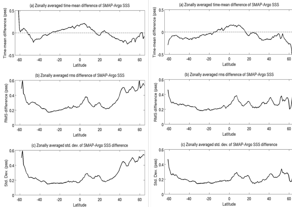
Figure 11: Comparison of zonally averaged statistics: time-mean difference, RMS, Standard Deviation of SMAP – ARGO SSS. Left: for V1.0 (BETA). Right: V2.0. Provided by T. Lee, JPL.
