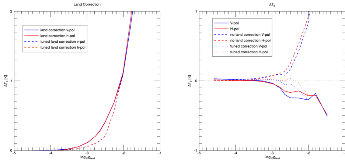
Figure 6: Left: Land correction for V1.0 (full lines) and V2.0 (dashed lines). Right: TA measured minus expected using the land correction in V1.0 (full lines), using no land correction (dashed lines) and using the mitigated land correction in V2.0 (dotted lines).
