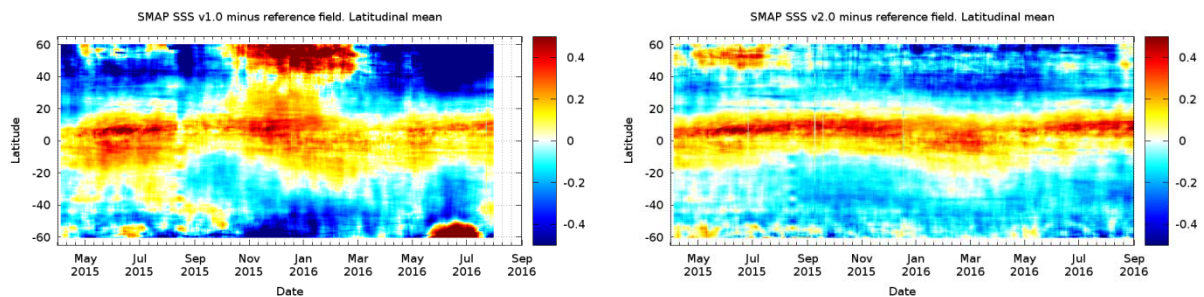
Figure 8: Latitudinal mean SMAP SSS – FOAM SSS. Left: V1.0 (BETA). Right: V2.0. Provided by J. Martínez, BEC.
