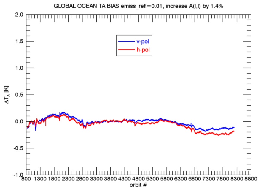
Figure 7: Running 3-day averages of TA measured – expected v-pol and h-pol over the open ocean.
