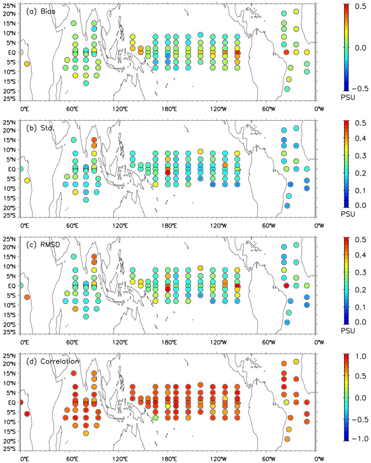
Figure 4.3: Comparison of SMAP SSS with salinity measured by moored buoys at 1 m depth: (a) Biases, (b) standard deviation, (c) RMS difference and (d) correlation coefficients.
