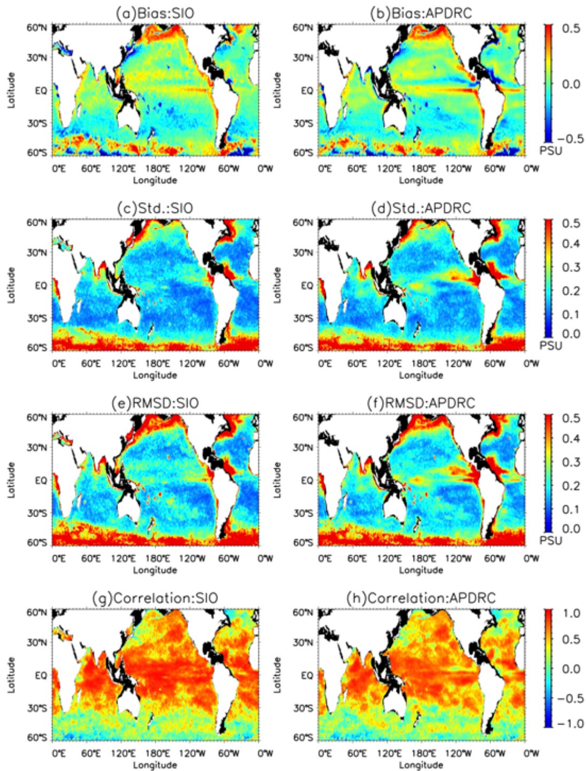
Figure 4.1: Comparison of SMAP SSS V4.2 with the monthly gridded Argo product from SIO (left) and APDRC (right): (a & b) Biases, (c & d) standard deviation, (e & f) RMS difference and (g & h) correlation coefficients for the period from April 2015 to December 2019.
