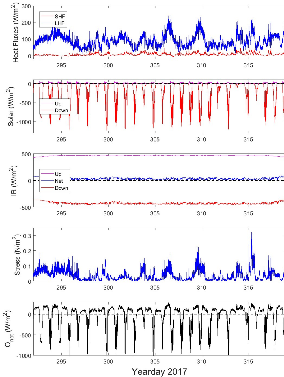
Figure 3. Heat budget terms and the surface stress as a function of Yearday 2017 during the Fall recovery cruise. The data represent 1 minute averages. The sum of the radiative and heat flux terms provide an estimate of the net heat flux, Q_{net} , as shown in the lower panel.
