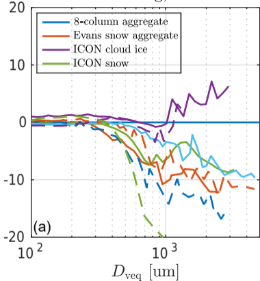
Back-scattering, 94.1 GHz
