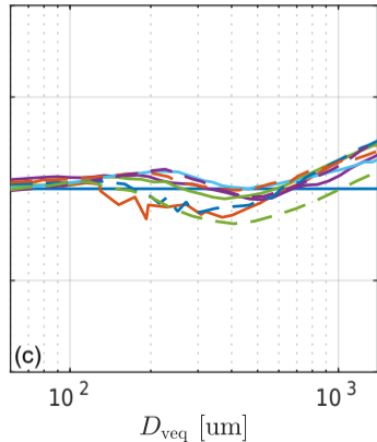
Extinction, 668.2 GHz
