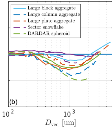
Extinction, 190.31 GHz
