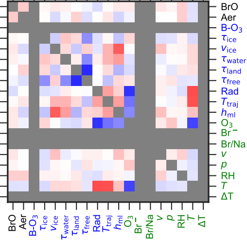
(f) FMA
