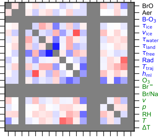
(f) FMA
