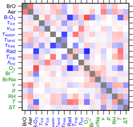
(e) FMA
