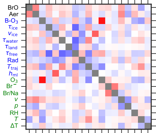
(e) FMA
