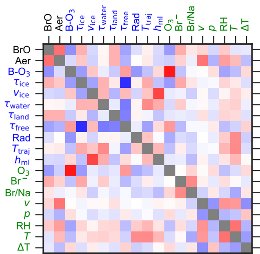
(c) NDJ
