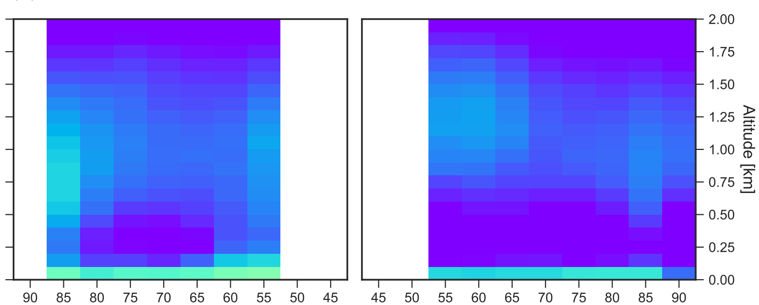
(f) AH - BrO diurnal variation - FMA
