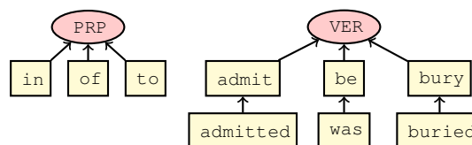
Figure 5: Items Hierarchy
