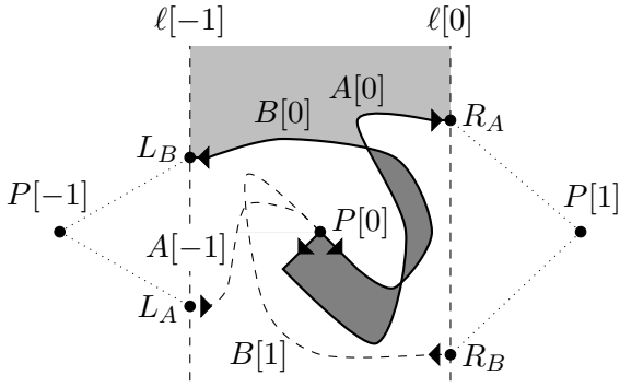
Figure 13: The region between \ell[-1] and \ell[0] is divided by A[0] and B[0] into a ‘top’ region (lightly shaded), a ‘bottom’ region (white), and areas enclosed by intersections of A[0] and B[0] (darkly shaded). Here A[-1] and B[1] are both in the ‘bottom’ region.
