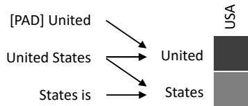
(a) An example of multigranular interaction over different n -grams (2:1).
