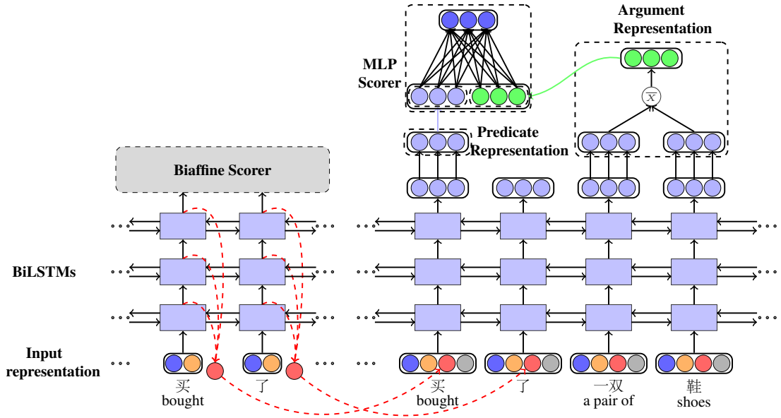
Figure 2: The detailed architecture of our proposed framework, where the left part is the dependency parser and the right part is the basic SRL module, respectively.
