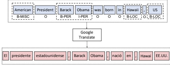
Figure 2: The Translate step of our method.
