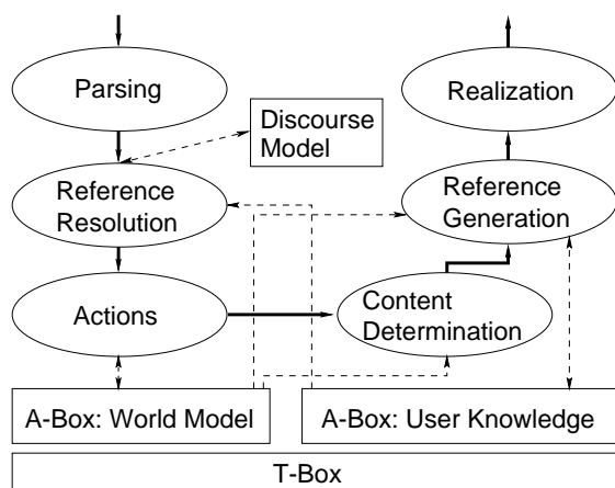
Figure 2: The architecture.
