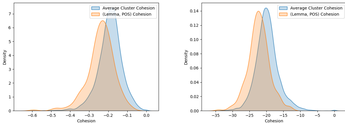
(b) Density function estimations for cluster and (lemma, PoS) cohesion when using cosine (left) and Euclidean (right) distances with DeBERTa as underlying encoder.
