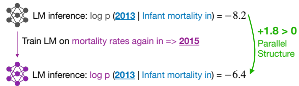
Figure 2: To measure the parallel structure strength of two phrases (c_f, x_f) and (c_l, x_l) , we take a pre-trained LM (gray), fine-tune it on x_f conditioned on its context c_f (purple), and measure the change in its predicted probability on x_l conditioned on context c_l (blue).
