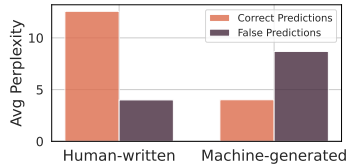
Figure 7: Comparison of the average perplexity of texts which the Longformer detector predicts correctly and incorrectly.
