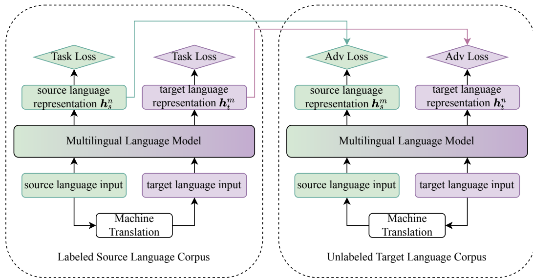
Figure 1: Overall cross-lingual information extraction framework
