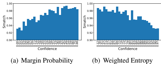
Figure 3: Diagrams for the model’s confidence versus SMATCH scores on the test set. Each bin contains 50 examples.
