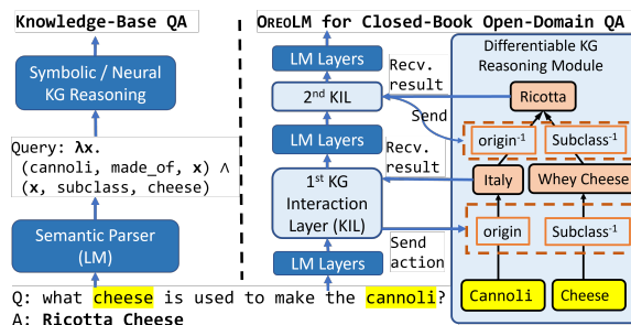
Figure 1: An Illustrative figure of OREOLM. Compared with previous KBQA systems that stack reasoner on top of LM, OREOLM enables interaction between the two.
