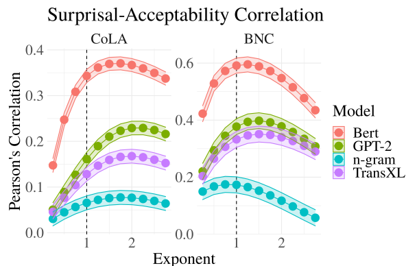
Figure 1: Correlation coefficient between (negative) sum of surprisals raised to the k^{\text{th}} power and linguistic acceptability judgments of a sentence. The higher correlation when k > 1 implies sentences with a more uniform distribution of information are more acceptable.
