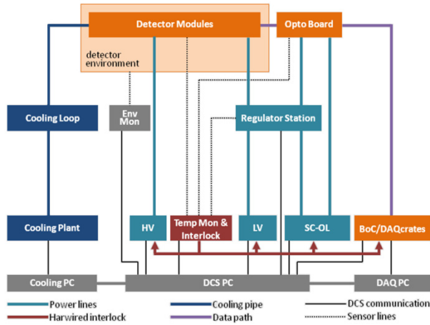
Figure 1: DCS Overview.
