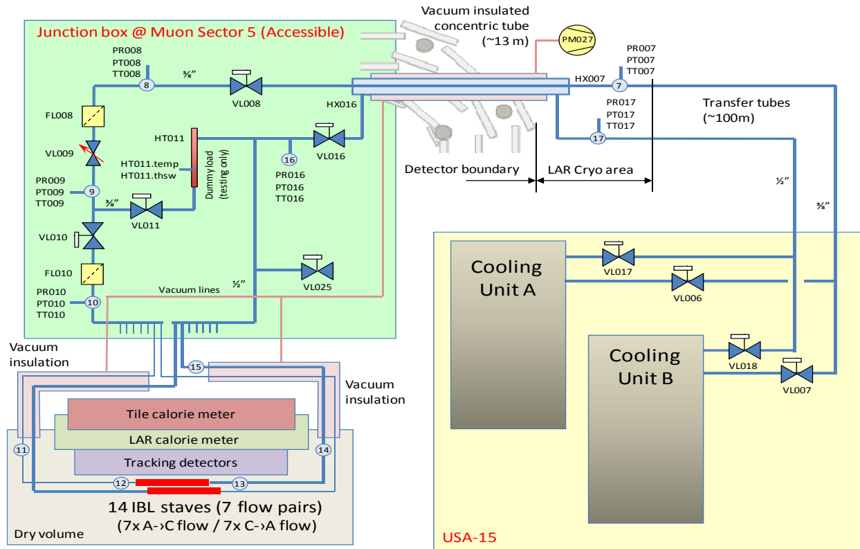
Figure 2: Cooling System.
