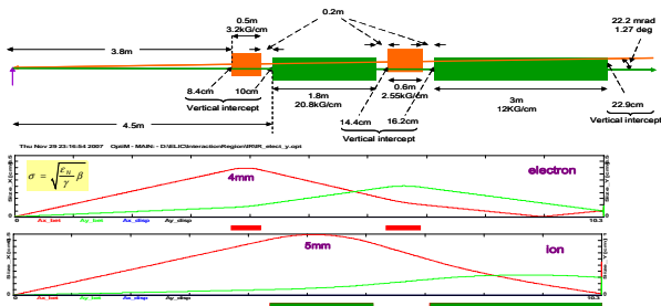
Figure 4. Layout and optics of an ELIC IR.
