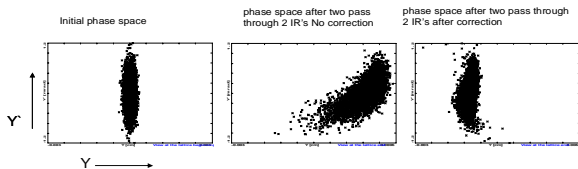
Figure 6. Electron vertical phase space distribution after two passes of an IP without and with sextupole correction.
