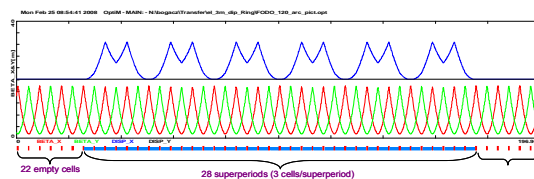
Figure 2. ELIC electron collider ring Lattice.
