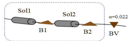
Figure 7. A prototype of arc-to-IR spin rotator for the ELIC electron ring.
