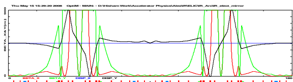
Figure 5. Electron optics around a pair of IRs -- Twiss functions with a confined vertical dispersion.
