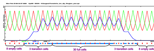
Figure 3. ELIC ion collider ring lattice.
