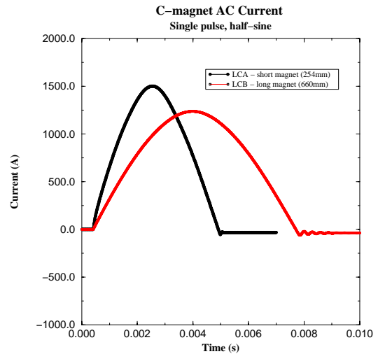
Figure 3: Current pulses used for the C-magnets
