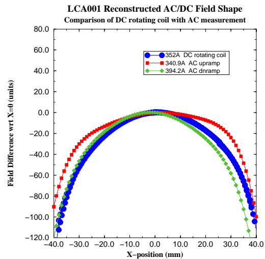
Figure 6: Field shape with no beam pipe. AC fixed probe data is shown compared to rotating coil at DC current.
