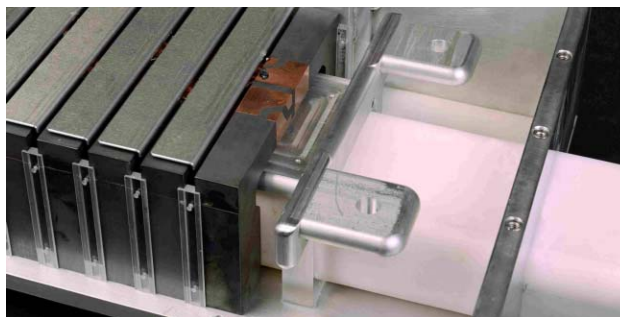
Figure 3: Recycler Ring kicker magnet.
