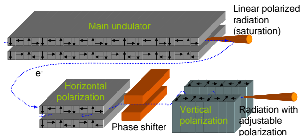
Figure 1: Modified crossed-planar undulator system for high-gain FEL generation.
