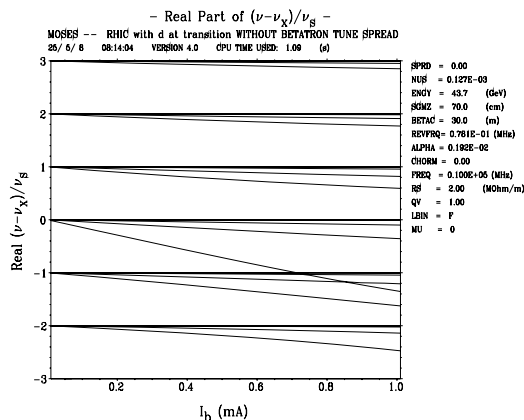
Figure 5: MOSES [9] output showing mode coupling for I_b = 0.7 mA, corresponding to 0.55 \times 10^{11} d /bunch, the instability threshold found experimentally without octupoles and zero chromaticity. A broadband impedance with 2 M \Omega /m and Q = 1 is used.
