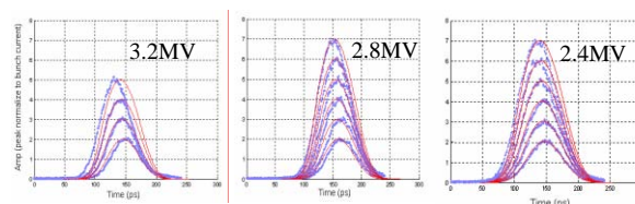
Figure 4: Haissinski curves for Q=0.7 model. Blue dots are raw data, solid red curves are fitted result.
