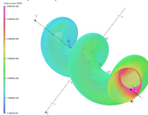
Figure 6: Helical Solenoid geometry and flux density for the Helical Solenoid magnet for MANX.
