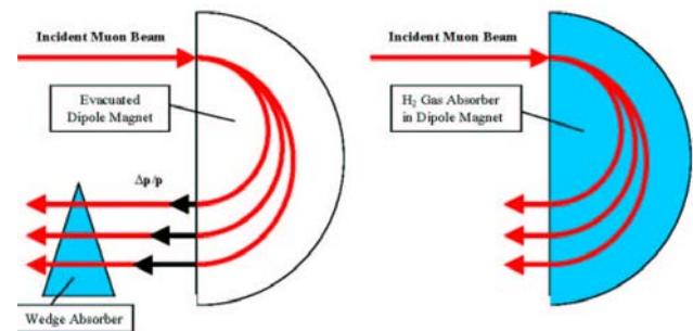
Figure 4: Emittance exchange. LEFT: Wedge Absorber Technique. RIGHT: Homogeneous Absorber Technique.
