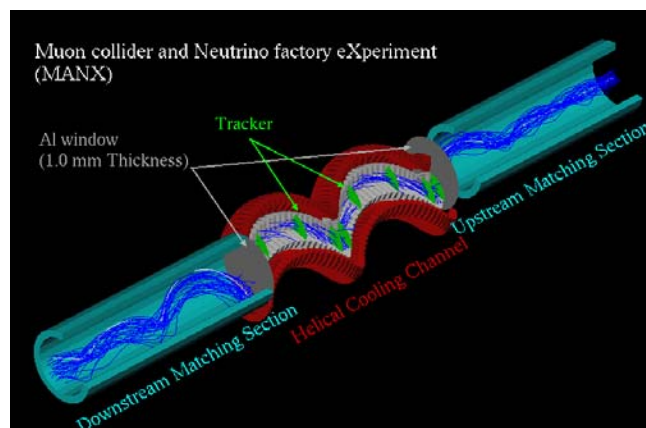
Figure 7: Conceptual picture of the MANX apparatus. The helical solenoidal magnets shown in red enclose the LHe ionization energy absorber, which is separated from the vacuum of the matching sections by thin Al windows.
