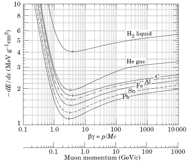
Figure 3: Energy loss for muons in various materials taken from the Particle Data Group [12], where the minimum dE/dx for hydrogen occurs near 300 MeV/c.
