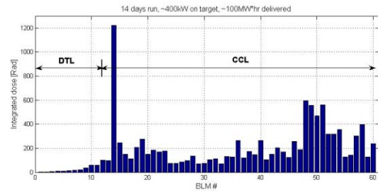
Figure 6 Measured distribution of prompt radiation due to beam loss in the warm linac.
