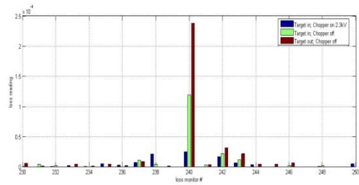
Figure 3 Effect of the MEBT chopper on the ring extraction losses. Bar chart is BLM readings: the brown bar– chopper is off, target is out; the green bar – chopper is off, target is in; the blue bar – chopper is on, target is in.
