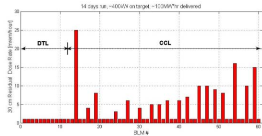
Figure 7 Measured distribution of the residual radiation in the warm linac after 36 hours of cool down period.
