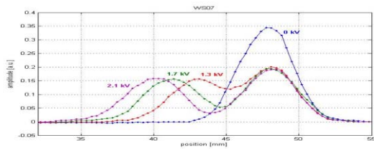
Figure 1. Vertical beam profile measured near the MEBT chopper target for different chopping voltages. Separation of two peaks in the profile is defined by the chopper kick strength.
