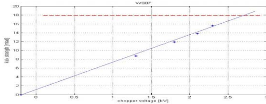
Figure 2 Chopper kicker strength vs. kicker voltage calculated from the profiles in Fig.1. Red dashed line shows the design requirements
