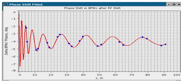
Figure 5. Synchrotron bunch oscillation in the DTL and CCL. Solid line is simulation result for the nominal cavity amplitudes; points are measured values for the case of good linac tuning.
