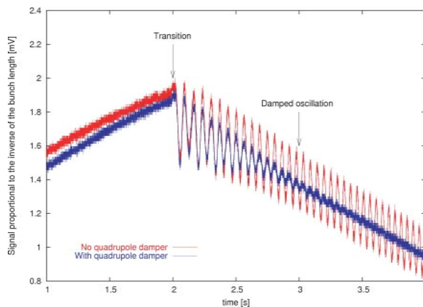
Figure 3: Amplitude of the WCM signal filtered at the fourth RF harmonic. This signal is proportional to the inverse of the bunch length, and is the averaged quadrupole motion of all 95 bunches stored in the machine. Without the feedback loop these oscillations persist for a period on the order of 10 seconds, while with the feedback loop closed they are damped in less than 1 second after transition.
