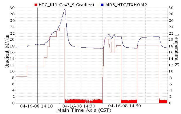
Figure 5: Runaway HOM coupler heating observed at 5 Hz for gradients > \sim 20 MV/m. The horizontal axis is a time span of about 1.5 hours. The red trace is the cavity gradient and the blue trace is a HOM coupler antenna temperature.
