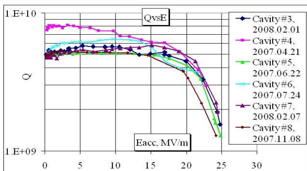
Figure 1: Vertical test results of the cavities #3-8. Cavity #4 was 120C 48hours baked.
