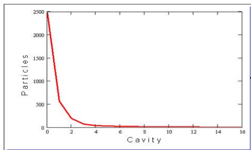
Figure 8: Number of dark current particles that reached upstream cavities. Only particles generated in cavity #0 are taken into account. In last four cavities 7 particles survived and captured in acceleration.
