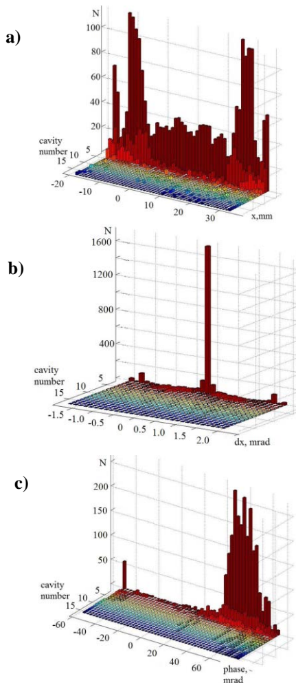
Figure 9: Distribution of the particles generated in cavity#0 at the entrance of each upstream cavity a) x -radial distribution; b) dx - angular distribution; c) phase distribution.
