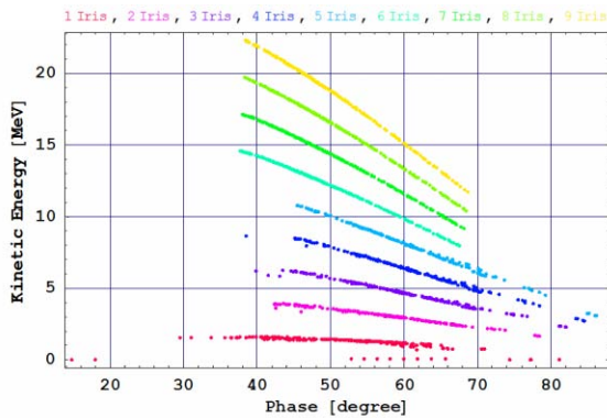
Figure 3: Kinetic energy of electrons vs. RF phase at the cavity exit. The points corresponding to different irises have different colors.
