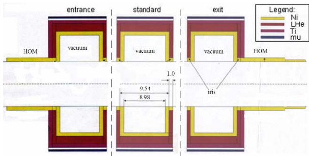
Figure 6: Simplified geometry of the 9-cell ILC cavity in MARS. Here only three cells are shown: input, middle (regular) and output.
