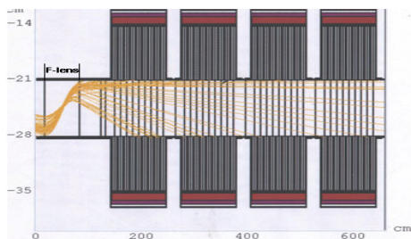
Figure 7: Trajectories of the survived dark current particles in focusing quad and followed 4 cavities.
