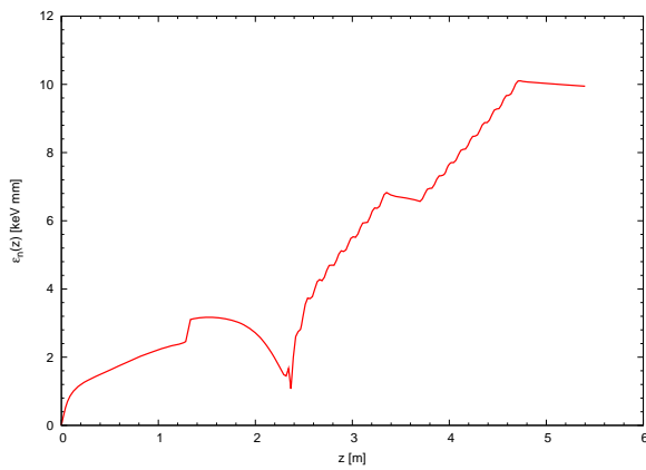
Figure 3: Longitudinal emittance.
