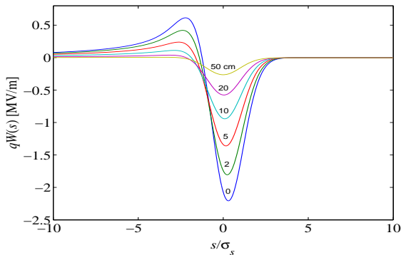
Figure 2: CSR exit wakefield at various distances (in cm) from exit of 50-cm long bend magnet (compare to Fig. 3 in reference [4]).
