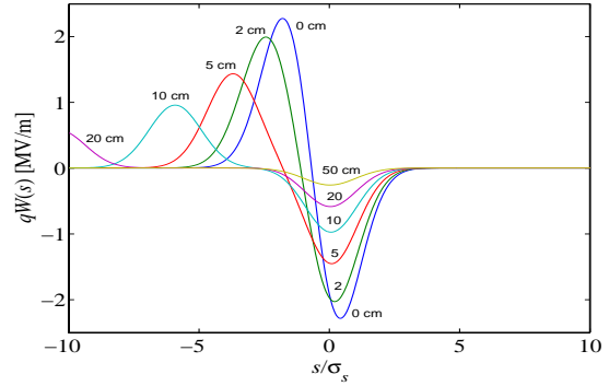
Figure 3: CSR exit wakefield at various distances (in cm) from exit of 10-cm long bend magnet with R = 1.5 m. In this case the bend-exit occurs before steady-state.
