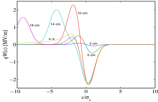
Figure 1: CSR entrance wakefield (times charge, q ) at various distances past bend magnet entrance (“s-s” is steady-state). Bunch head is at left (compare with Fig. 2 in reference [4]). Energy loss is at negative values here.
