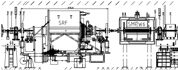
Figure2: SMPW6 locates at the down stream of the superconducting RF cavity.
