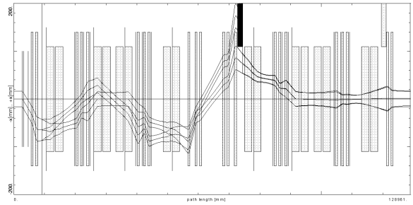
Figure 8: Fast extraction (high resolution mode)
