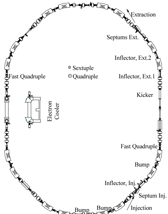
Figure 1: Layout of CSRm injection and extraction
