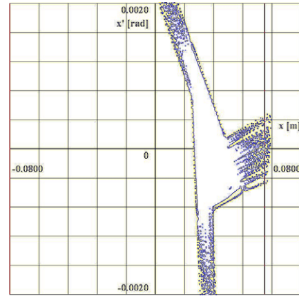
Figure 4: Tracking in real phase space
