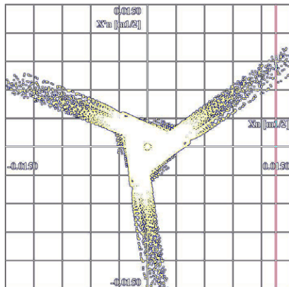
Figure 3: Tracking in normalised phase space
