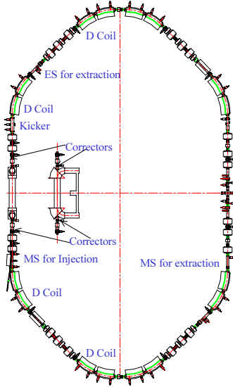
Figure 7: Layout of CSRe injection and extraction
