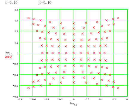
Fig2. Position map of calculation for cylindrical BPM
