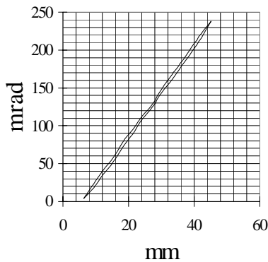
Fig3. Emittance plot of ion beam
