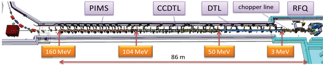
Figure 2: Linac4 layout.
