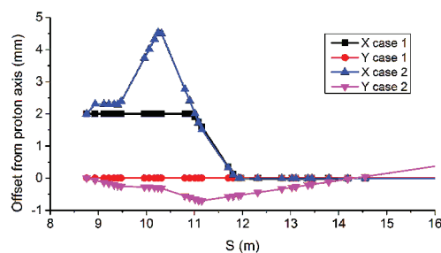
Figure 6: Beam trajectory of the electron beam injected into the common beam line with an offset for case 1 and 2.
