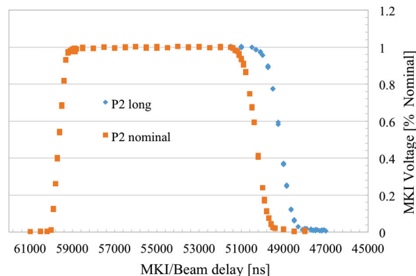
Figure 3: Nominal and long waveform of the MKI in IR2.
