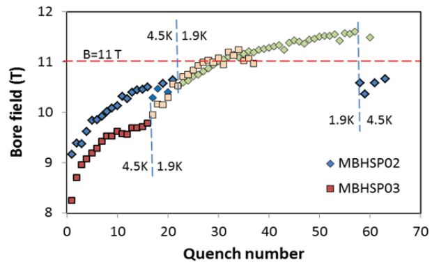
Figure 4: Magnet training.
