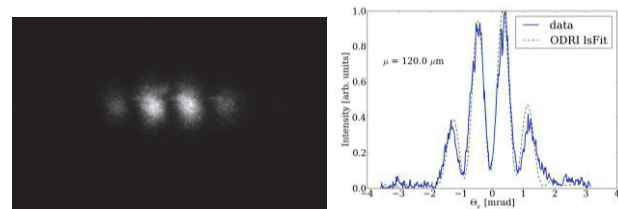
Figure 10: Image of DR angular distribution with mask/target interference case (left), and a least squares fitting 17.6 \mu\text{m} beam size, 4.08 \mu\text{rad} beam divergence and 0.12 mm beam offset w.r.t. the centre of the target aperture (right).
