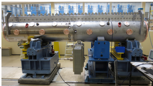
Figure 6: Drift tube linac tank 1.
