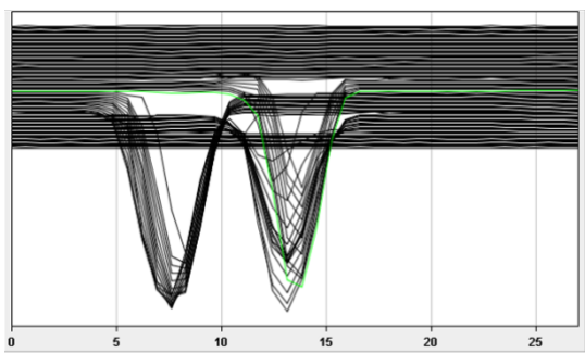
Figure 5: Transverse beam profile along the beam pulse after the chopper; chopped and main beam are fully separated.
