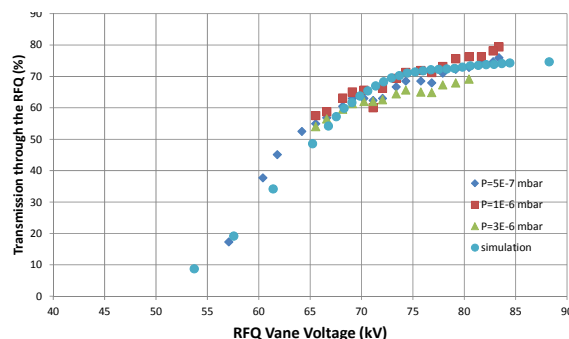
Figure 3: Transmission through the RFQ as a function of RF power.
