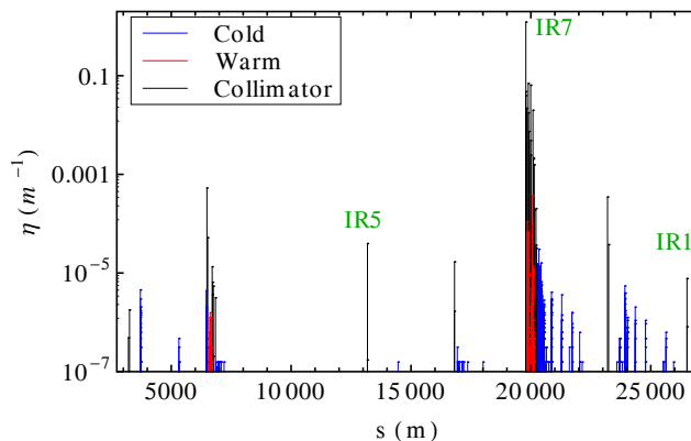
Figure 1: Cleaning inefficiency \eta (ratio of local losses per metre to the total losses on the TCPs), simulated with SixTrack, for the 2010 LHC running conditions (3.5 TeV, \beta^* = 3.5 m). The horizontal TCPs in IR7, beam 1, were hit first by the halo. The leakage to the TCTs in IR1 and IR5 is about 10^{-5} – 10^{-4} . The colour codes indicate if the losses occur on a collimator or in a warm or cold element.
