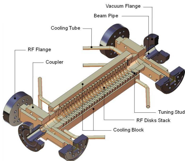
Figure 1: General view of the accelerating structure.
