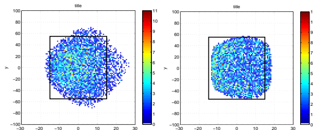
Figure 6: Beam halo x - y profile at the entrance of the FD before (Left) and after (Right) optimisation. In this example no beam energy spread has been considered. The black square contour represents the collimation window.
