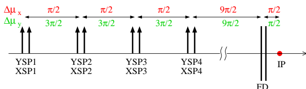
Figure 4: Schematic showing the approximate values of the phase advance between the CLIC betatron spoilers, FD and IP.
