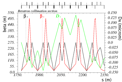
Figure 5: CLIC betatron collimation optics section.
