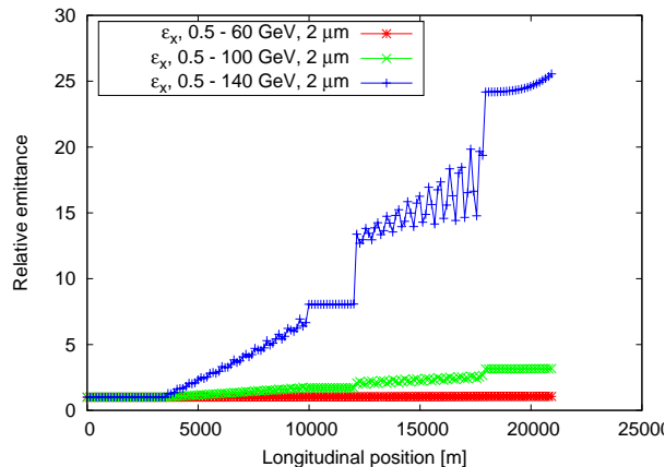
Figure 8: Relative emittance for three final beam energies (60 GeV, 100 GeV and 140 GeV), initial emittance is 2 \mu\text{m} .
