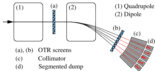
Figure 2: Sketch of a diagnostics section at TBL.
