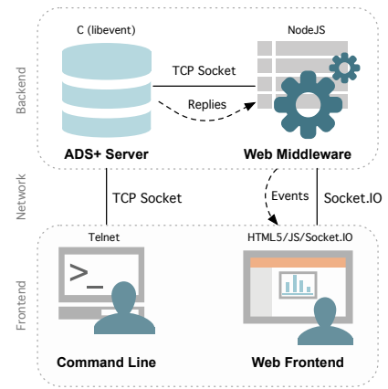
Figure 4: RINSE Architecture
