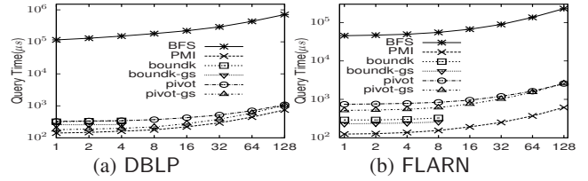
Figure 13: Query Time in Microseconds by Varying k
